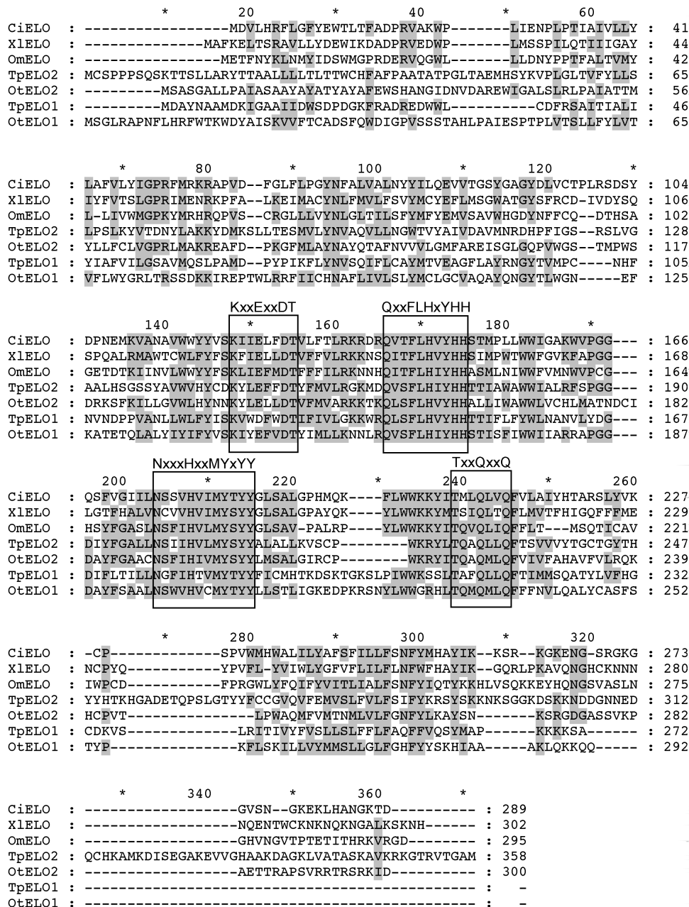
Fig. 2. Amino acid sequences of elongases characterized in the present study. The alignment was obtained using the CLUSTAL X program (gap opening 10, gap extension 0.05). Conserved amino acids are shown on a gray background, whereas conserved motifs found in all ELO-type sequences are framed. The nucleotide sequence data have been submitted to the DDBJ/EMBL/GenBank sequence data bank (see Table 2).
