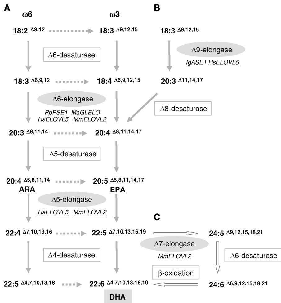
Fig. 1. \omega 6 and \omega 3 pathways for the synthesis of long-chain polyunsaturated fatty acids in eukaryotes. \omega 6-18:2 and \omega 3-18:3 can be converted to docosahexaenoic acid (DHA) by the consecutive action of desaturases and elongases, either starting with a \Delta 6 desaturation (A) or with a \Delta 9 elongation (B). In mammals, the \Delta 4 double bond in DHA is the result of a more complicated series of reactions that involve the elongation to a C24 fatty acid, a second \Delta 6 desaturation, and the final chain shortening in peroxisomes (the so-called Sprecher pathway; C). \omega 3-desaturases (dashed arrows), which link the \omega 6 and \omega 3 pathways in many eukaryotes, are missing in mammals. Examples of cloned elongases involved in DHA synthesis have been included in the figure. Although some elongases are specific for a single step (e.g., the moss PpPSE1 and the fungal MaGLELO ), others are nonspecific or multifunctional and show up at several steps (e.g., the human HsELOVL5 and the murine MmELOVL2 ; underlined).
