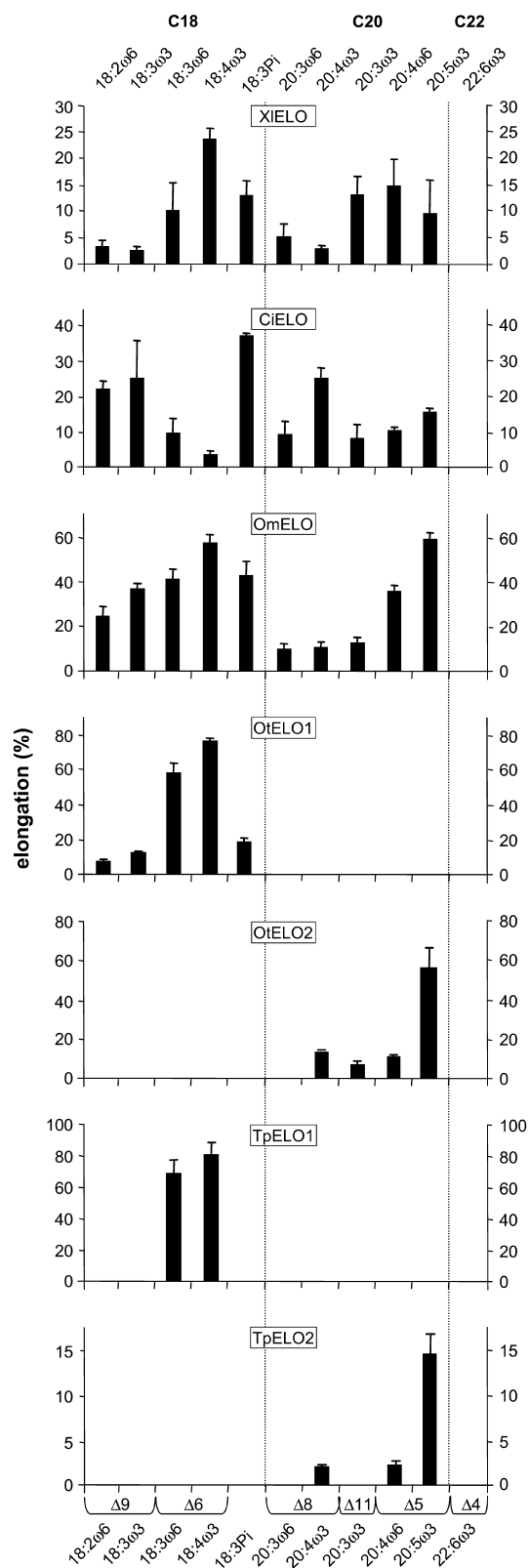
Fig. 4. Specificities of functionally expressed elongase enzymes. All transformed yeasts were separately incubated with 250–500 \mu\text{M} of the C18, C20, and C22 fatty acids listed on the abscissa for 4 days, except for pinolenic acid [18:3 \Delta^{5,9,12} (18:3Pi)], which was part of a fatty acid mixture isolated from Larix seeds. Fatty acid profiles were analyzed by gas-liquid chromatography. The elongation is given as [product/(substrate + product) \times 100]. Each value is the mean \pm SD from three to five independent experiments.
